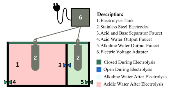
Figure 1. Design of a Simple Household-Scale Electrolysis Device
