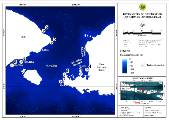
Source: Research results, 2025 Figure 5. Bathymetry Map of Lombok Strait
