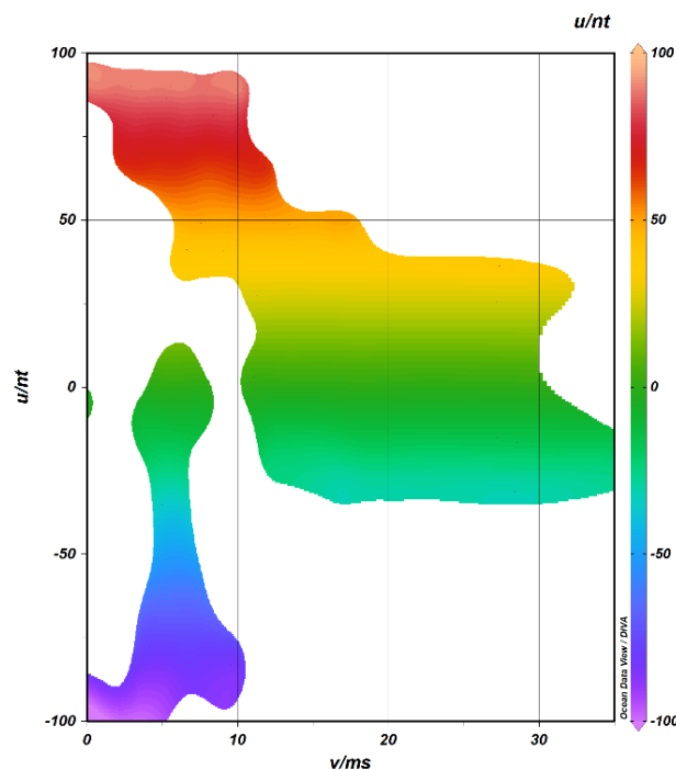
Figure 4. Filled Contour Current Plot ODV Bali Sea - Indian Ocean
