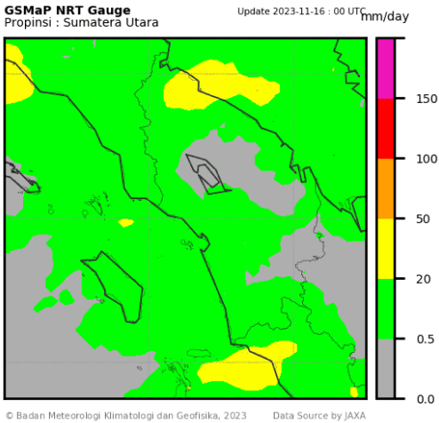
Figure 16. Daily North Sumatra Precipitation 16 November 2023
