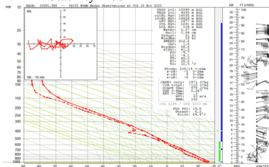
Figure 14. Kualanamu Class I Meteorological Station radiosonde 16 November 2023 00 UTC
