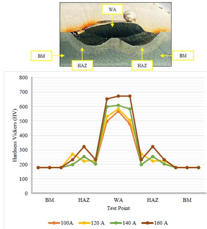
Figure 7. Vickers Hardness Graph
