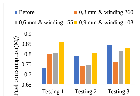
Figure 12. Average Test Results Fuel Consumption
