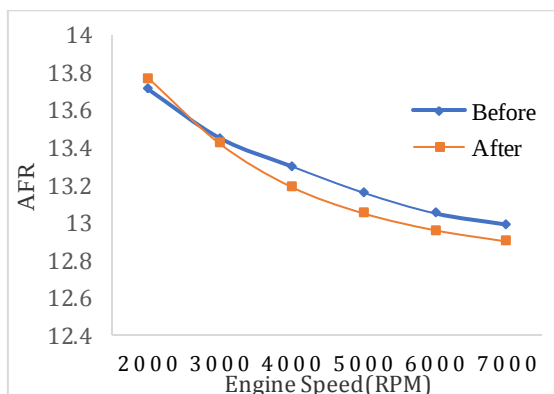
Figure 11. AFR engine uses groundstrap 0.9 with winding 103
