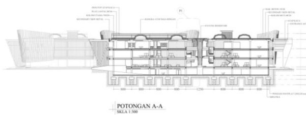
Figure 24 Section A-A
