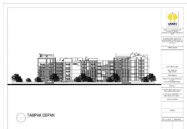
Figure 9 Front Elevation
