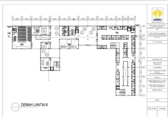
Figure 10 6th Floor Plan
