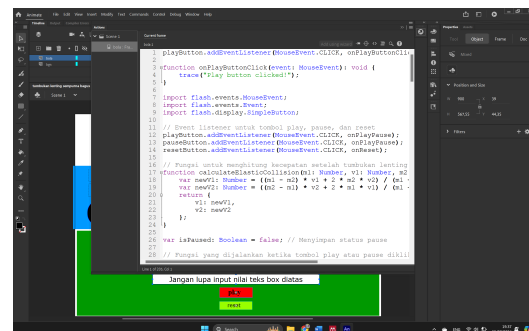
Figure 3. Collision algorithm implementation in action script 3.0
