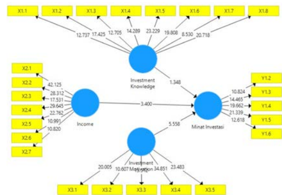
Figure 3. Bootstrapping
