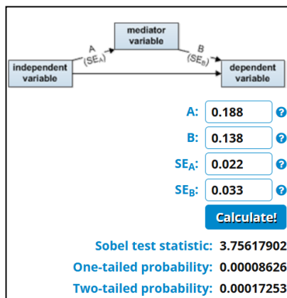
Figure 4. Sobel test
