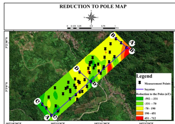
Figure 5. Magnetic anomaly contours after reduction to poles
