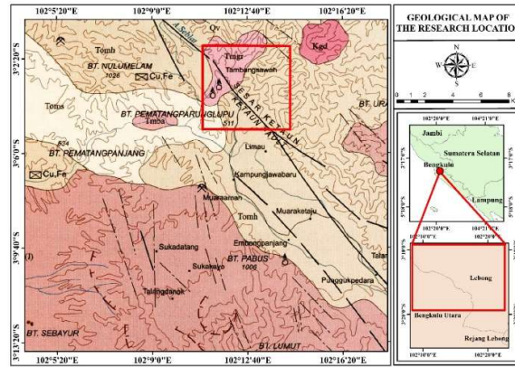
Figure 1. Regional geologic map of Lebong Regency
