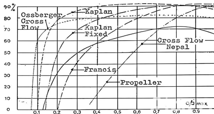
Figure 3. Turbine efficiency diagram
