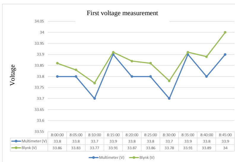
Figure 7. First Voltage Test Graph of the Monitoring System
