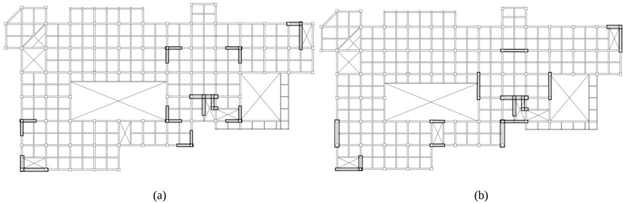
FIGURE 2. Building Plan Configuration with Shear Wall (a) M2 and (b) M3
