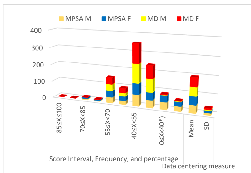
Figure 4. Visualization of MPSA and MD test scores by gender
