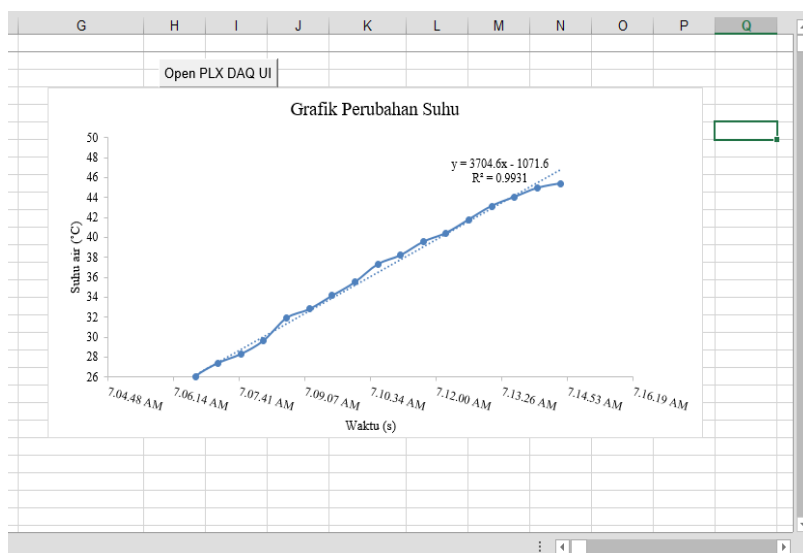
Figure 6. Display of temperature reading results in graphic form from PLX-DAQ software in Microsoft Excel
