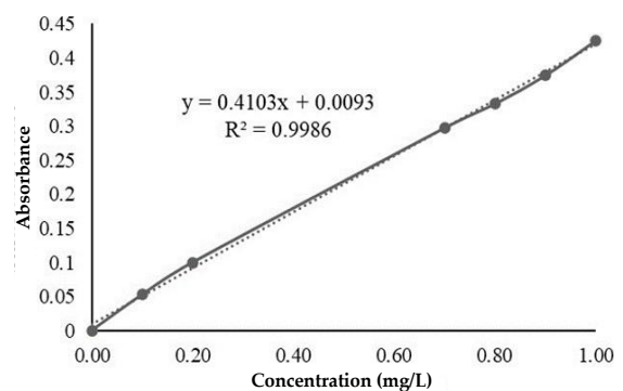
Figure 2. Standard Potassium Calibration Curve
