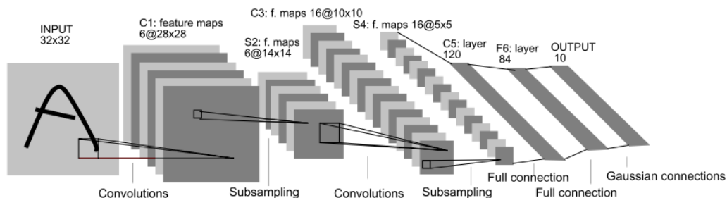
Figure 2. Architecture of LeNet-5 [18]
