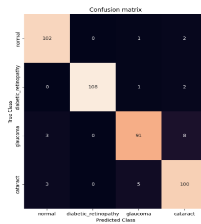
Figure 6. Confusion Matrix Fine-Tuning
