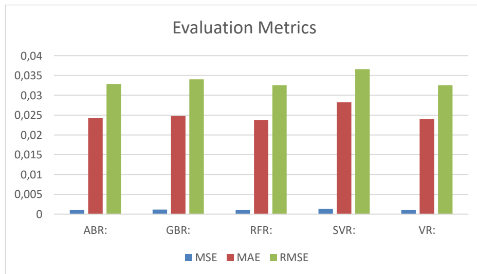
Figure 3. Evaluation metrics
