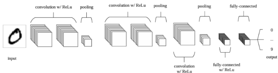
Figure 3. CNN structure [31]
