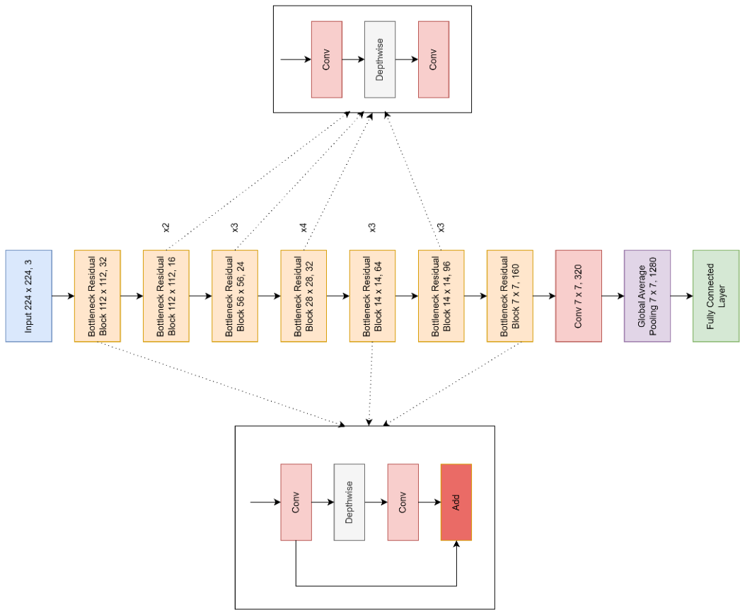
Figure 4. MobileNetV2 architecture
