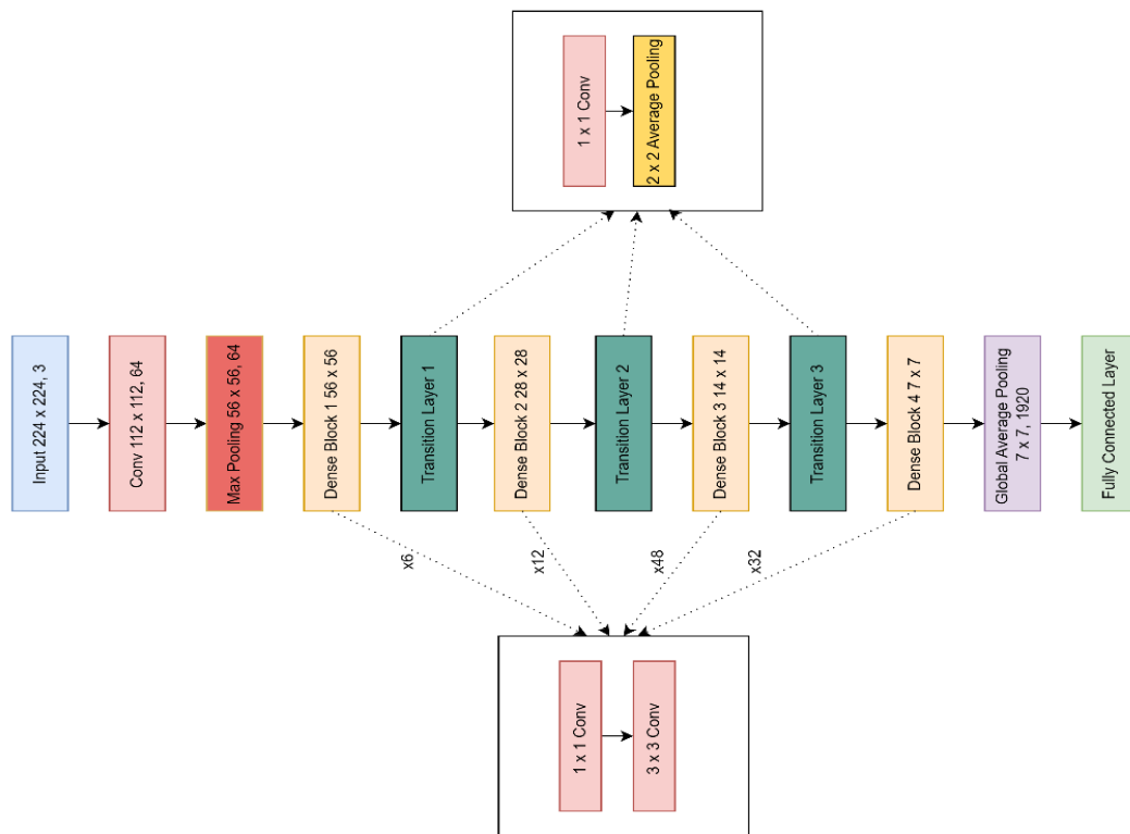
Figure 5. DenseNet201 architecture
