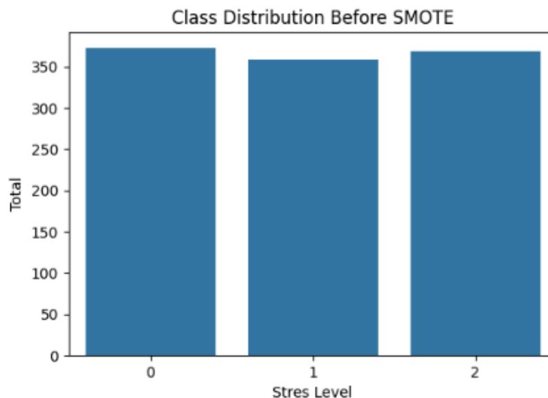
Figure 2. Class distribution before SMOTE
