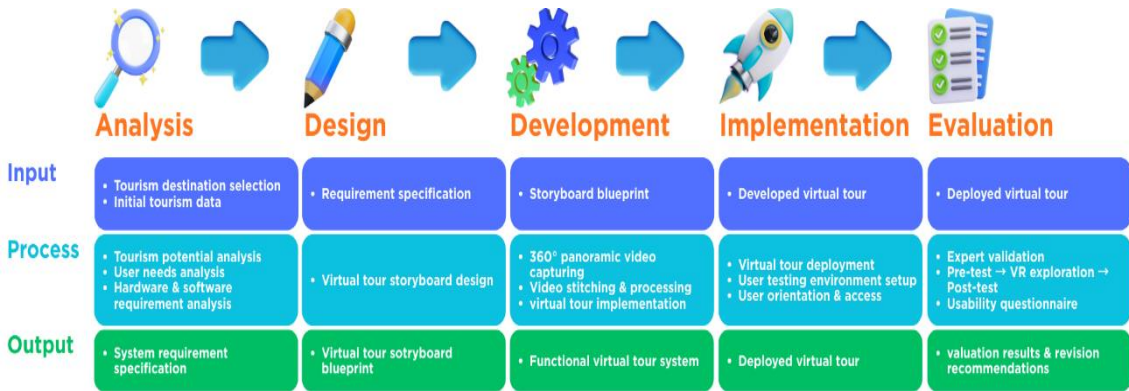
Figure 1. Research Method
