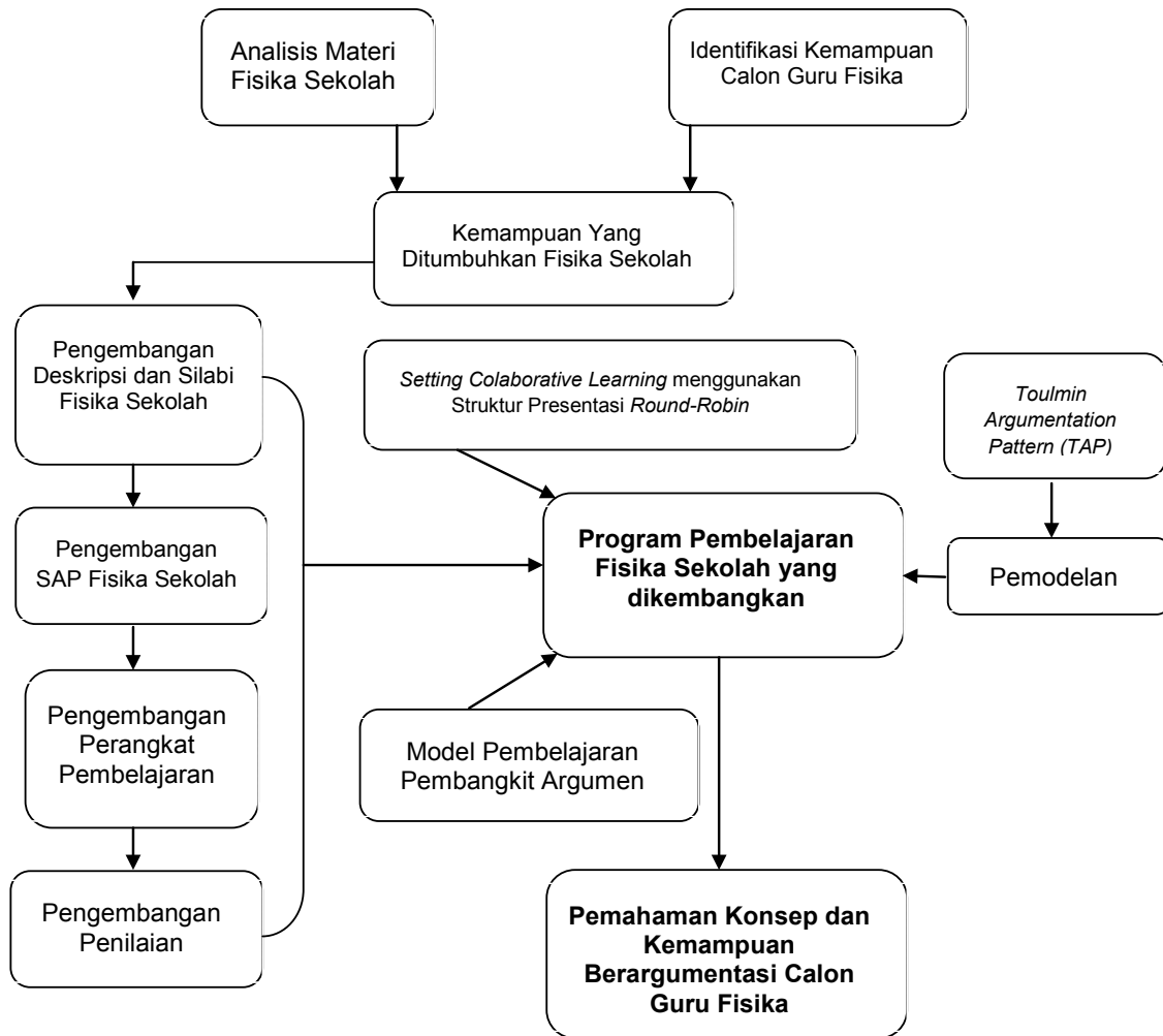
Gambar 1. Paradigma Penelitian
