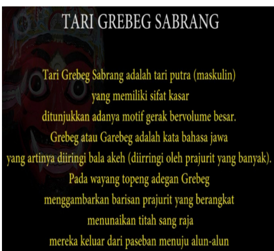
Gambar 4. Tampilan Synopsis
