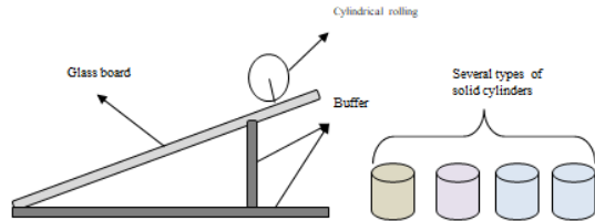
Figure 5. Tools design for determination swipe coefficient on cylinder solid material
