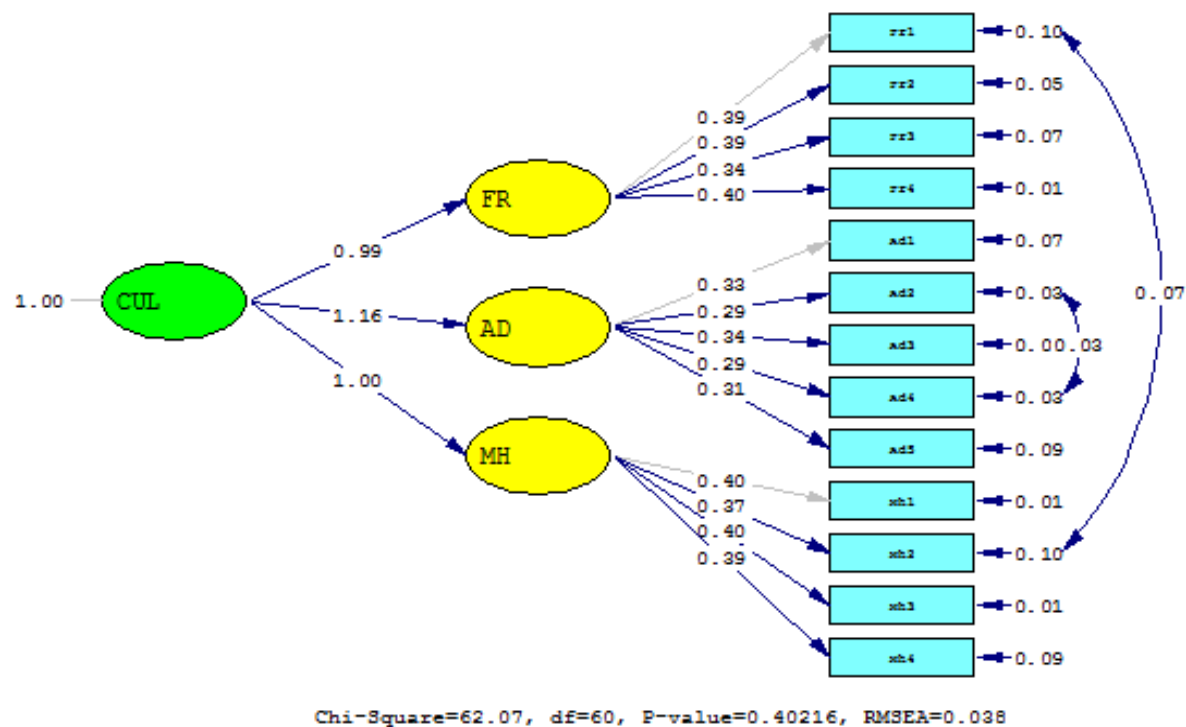
Figure 1. Conceptual model ( standardized solution ) of school cultures
