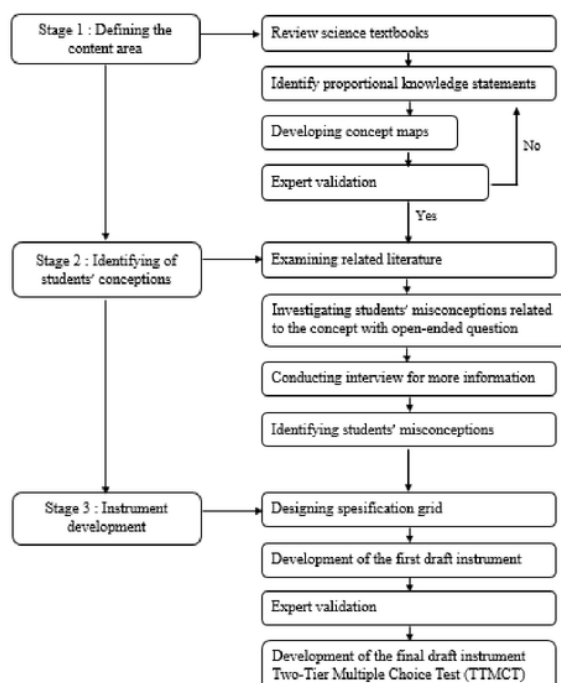
Figure 1. The flowchart of instrument development based on Treagust (1988,1955)
