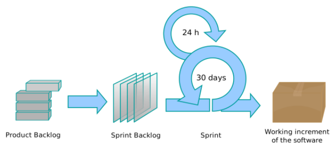
Gambar 1. Scrum process
