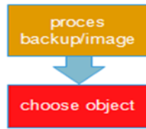
Figure 4. Process analysis
