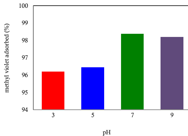
Figure 6. The effect of pH toward methyl violet adsorbed (Initial concentration of 50 mg/dm -3 , time of 90 minutes, dose of adsorbent of 2gr/100cm -3 solution)
