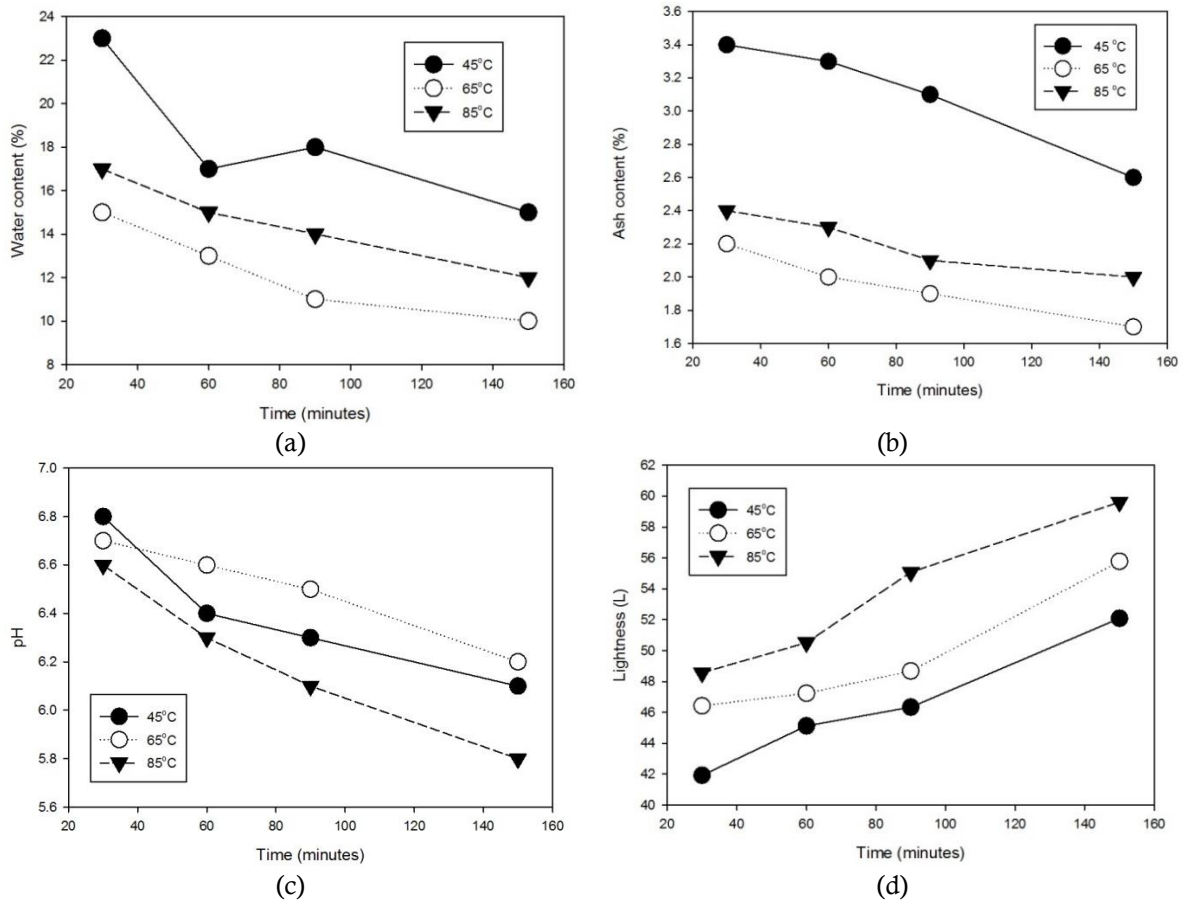
Figure 3. Effect of time and temperature of demineralization on (a) moisture content, (b) ash content, (c) pH and (d) Lightness (L)
