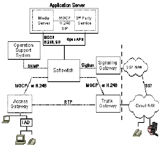
Gambar 3. Protokol-Protokol Softswitch
