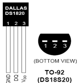
Gambar 1. Sensor Suhu DS18S20 TO-92
