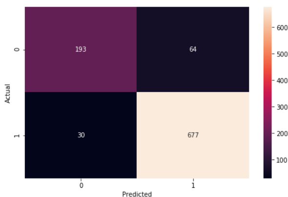
Figure 3. Visualization of confusion matrix result
