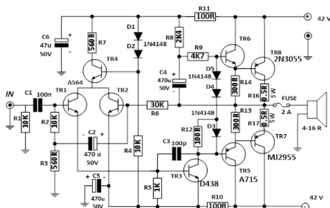
Gambar 7. Power Amplifier
