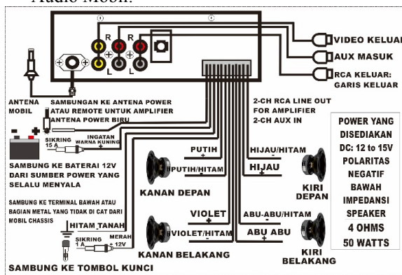
Gambar 4. Wiring Diagram Head Unit SN-5217
