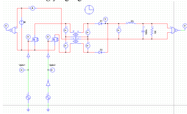
Gambar 5. Simulasi Power Supply Switching
