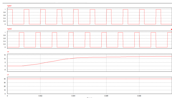
Gambar 6. Sinyal Output Power Supply Switching
